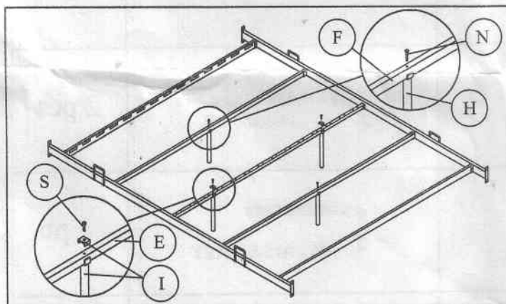
Step 3 Fix bed support legs as shown on the picture.
