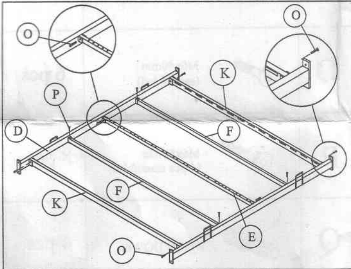
Step 2 Fix both side rails and cross bar E with bolt O as above diagram. Put cross bar F into side rail and fix in bolt P. After that put end cross bar K to the end of side rail and tighten with bolt O.
